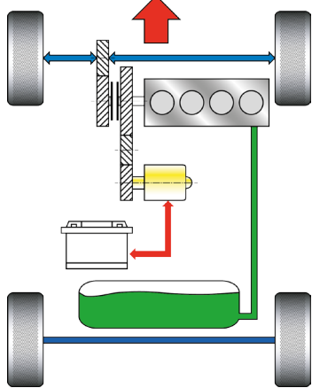
P1 Parallelhybrid
