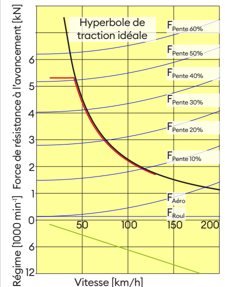
Diagramme de traction d'un BEV (Battery Electric Vehicle)
